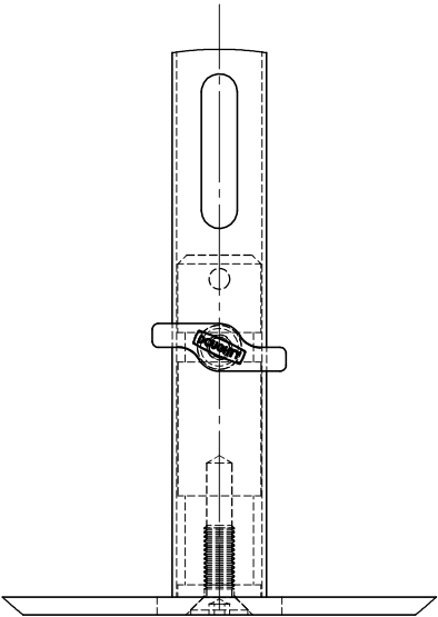
DETAIL A SCALE 1 : 2
