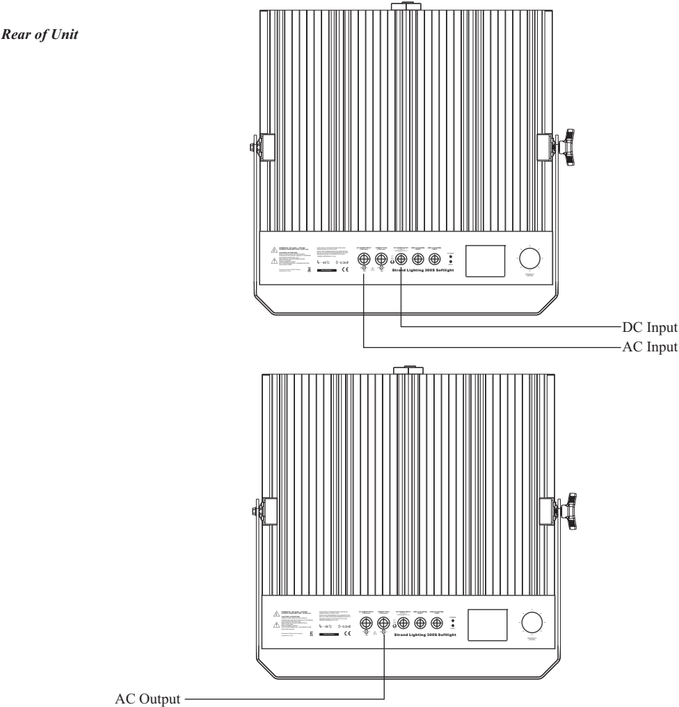
Figure 3: 300S Softlight LED Luminaire AC Input & Output Connections
