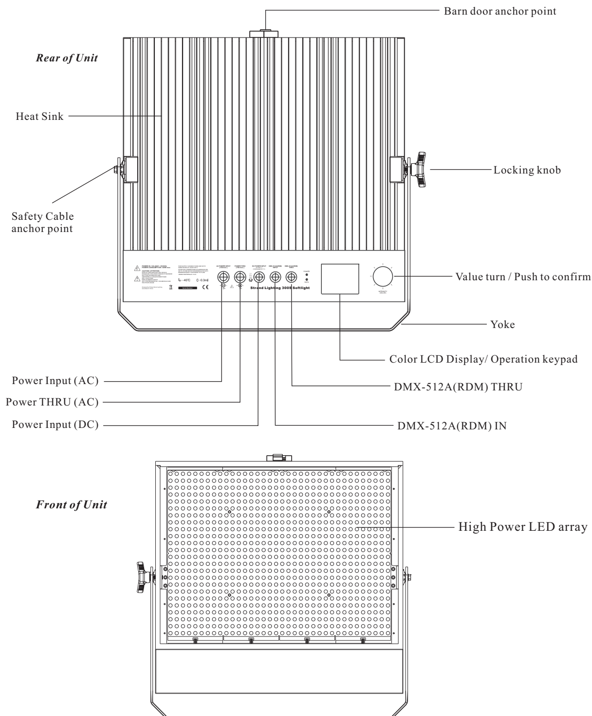
Figure 1: 300S Softlight LED Luminaire Components
