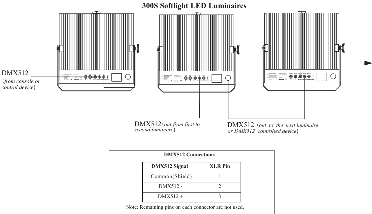
Figure 5: 300S Softlight LED Luminaire - DMX512 Connections
