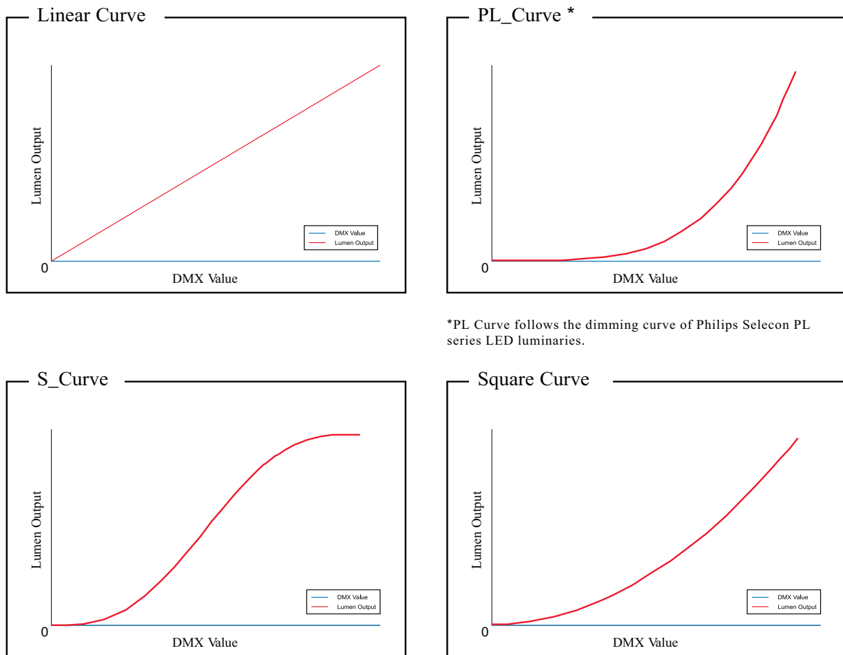
Figure 9: 300S Softlight LED Luminaire Dimmer Curves
