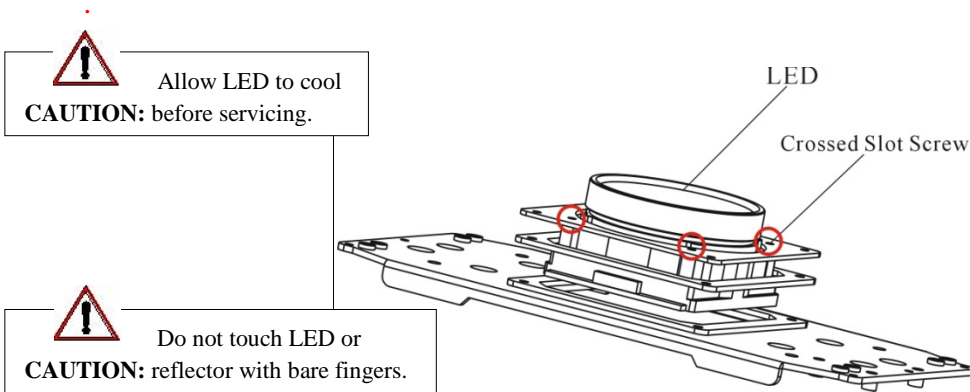
Figure A-1: Installing LED
