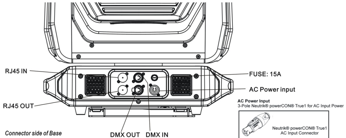
Figure 2-1: Power Connector
