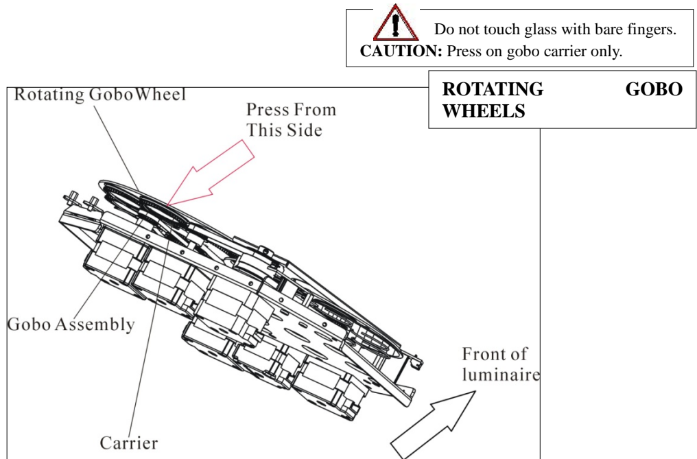
Figure A-3: Replacing Gobos
