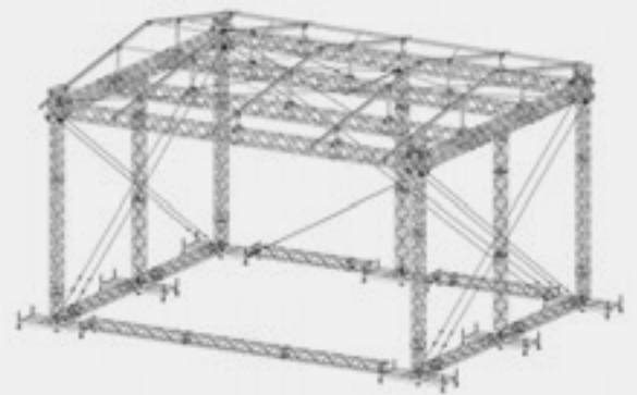
3D view
