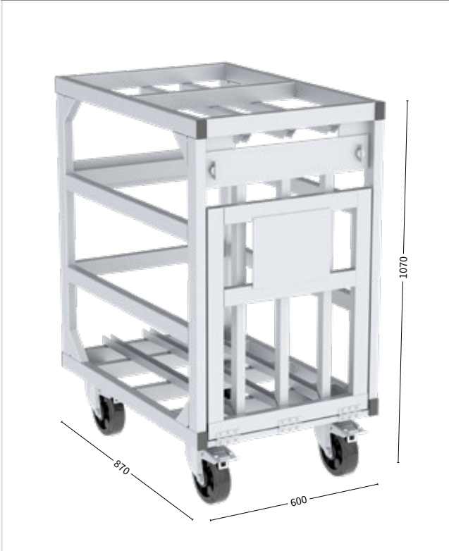
Dolly for 6 baseplates 80 cm round 215011
