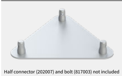
BASE PLATE 211005 429 x 384 x 5 mm
