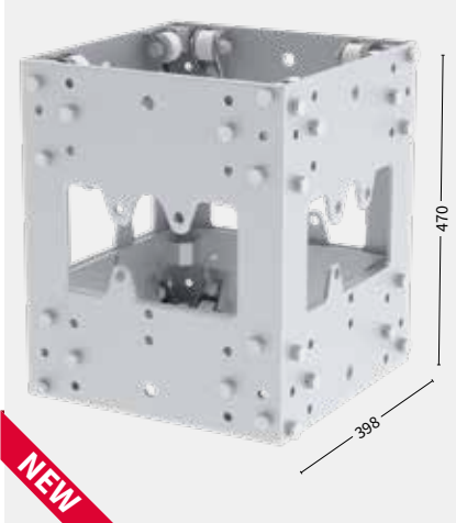
SLEEVE BLOCK PLATED M10 232001 25.2 kg
