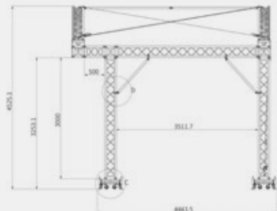
Left view
