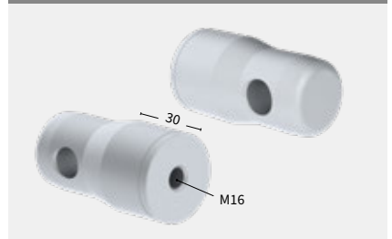
HALF CONNECTOR 203002
