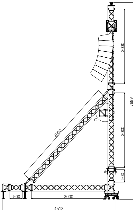
Right view
