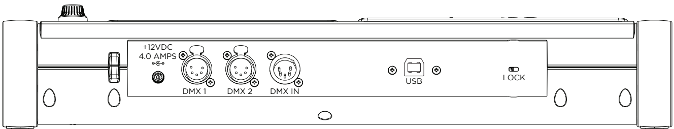
FIGURE 2. CONNECTIONS
